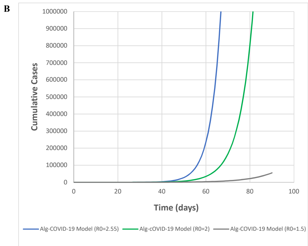
Fig. 1. A: Alg-COVID-19 Model match to actual data (cumulative cases) of epidemic's first 26 days. B: Alg-COVID-19 Model before and before ( R_0=2.55 ) and after mitigation ( R_0<2.55 ).
